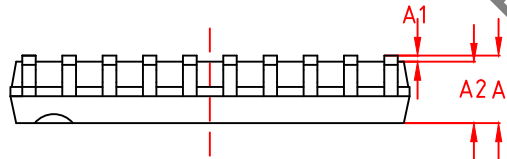
SIDE VIEW 侧视图
